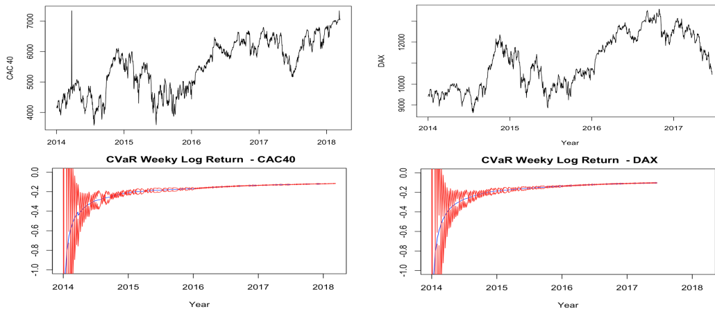
Figure 4: Convexified algorithm on Yahoo! Finance datasets.
