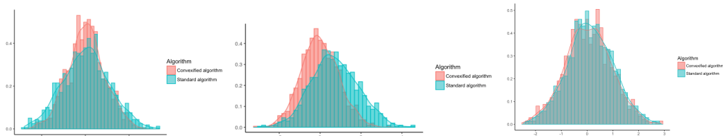
Figure 2: Distribution of the rescaled algorithms in different situations: left ( a = 2/3 < b = 4/5 < 1 ), center ( b = 2/3 < a = 4/5 < 1 ), right ( a = 2/3 < b = 1 ).
